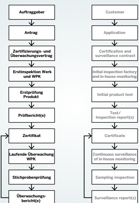
Schematic procedure of the product certification according to system 1+
